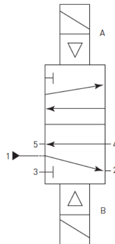
FIGURE 3 - DUAL COIL VALVE
