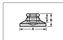
LF-M12-F Self Leveling Foot
