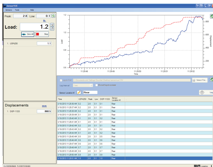
SensorVUE Force-Time Screen
