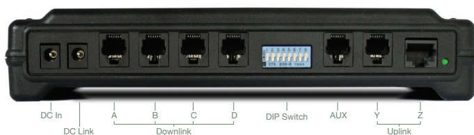
Back View
