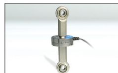
With Tension Adapter (TX-125) & Rod Ends (RE-125)
