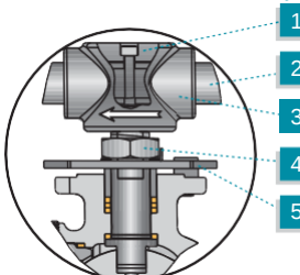
Manual Valve stem assembly
